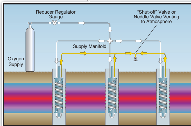
Multiple Well Installation with a Single Gas Supply
