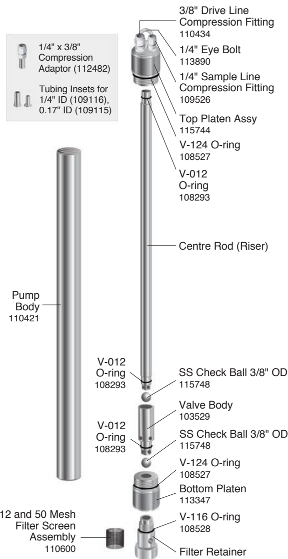
(Filter Retainer and Screen Assembly (Complete) 110517)
